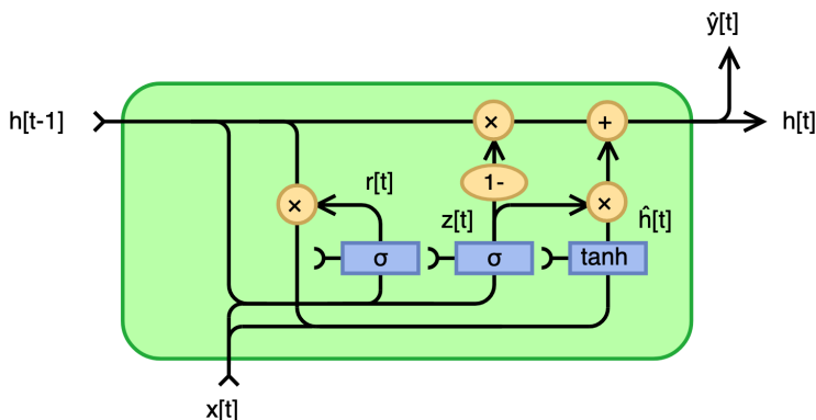
Figure 5: The computation for our GRU
