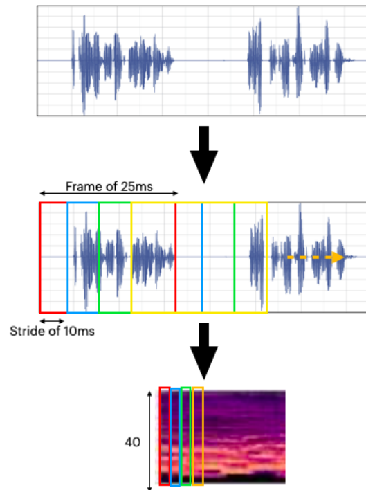
Figure 1: Feature extraction
