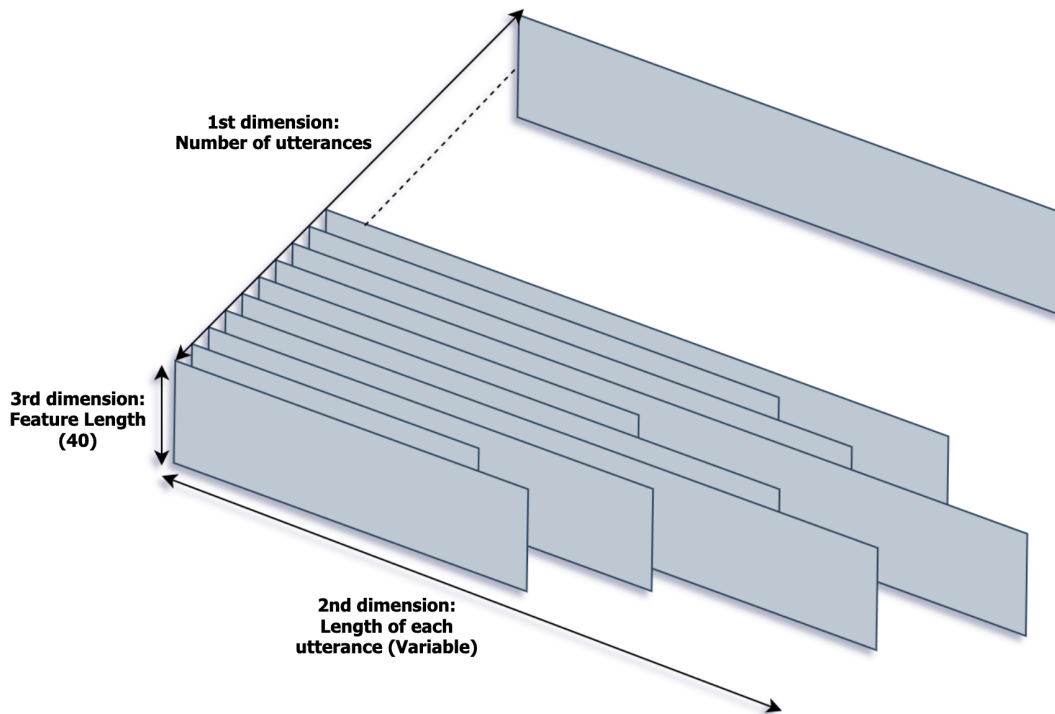
Figure 2: Data representation
