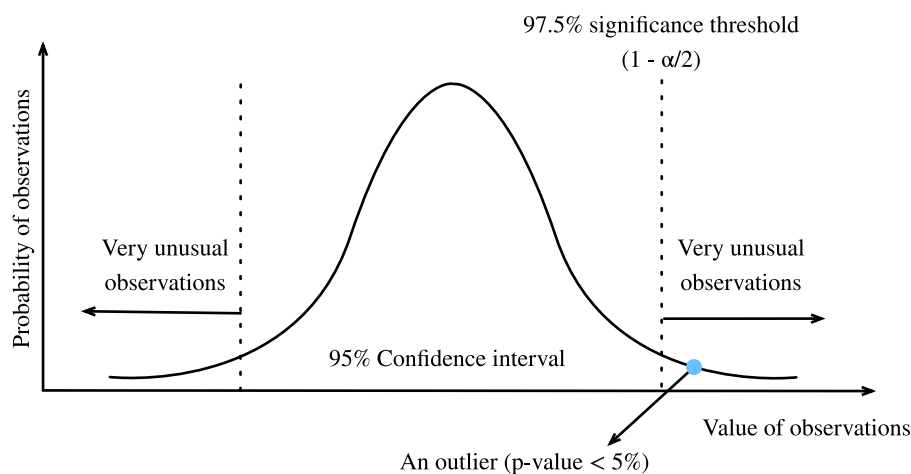
Fig. 18.10.1: Statistical significance.
