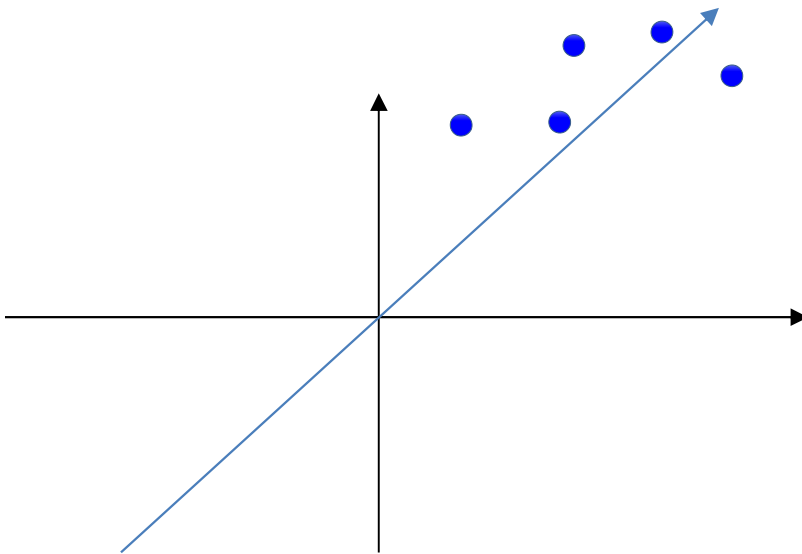
Karhunen Loeve Transform
