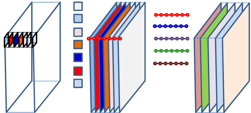
Depth-wise
