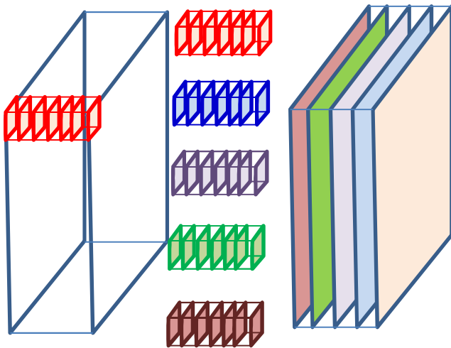
Conventional
