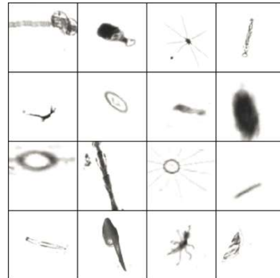
Augmented data
