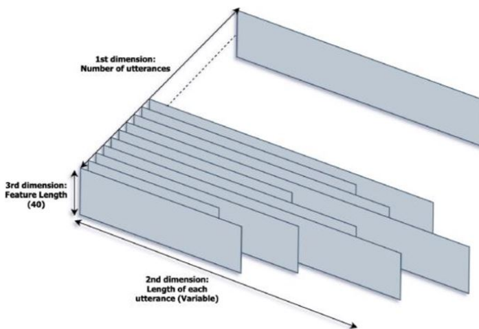
Figure 2: Data representation
